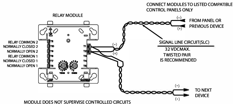
FIGURE 3. RELAY MODULE WIRING DIAGRAM
