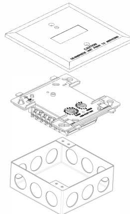
FIGURE 2. MODULE MOUNTING
