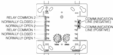
FIGURE 1. CONTROLS, INDICATORS, AND TERMINAL DEFINITIONS
