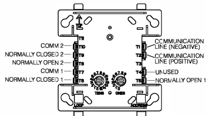
FIGURE 4. RETROFIT TERMINAL DESIGNATIONS FOR LEGACY FRM-1-AUS
