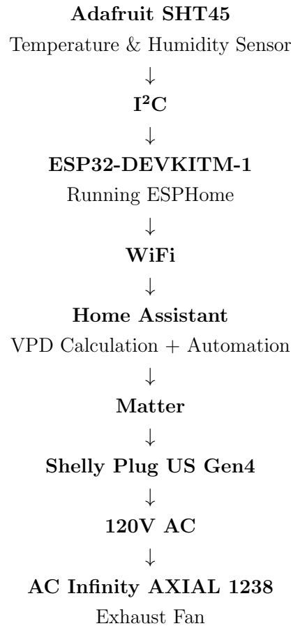
Figure 1: Proposed sensing and control architecture.
