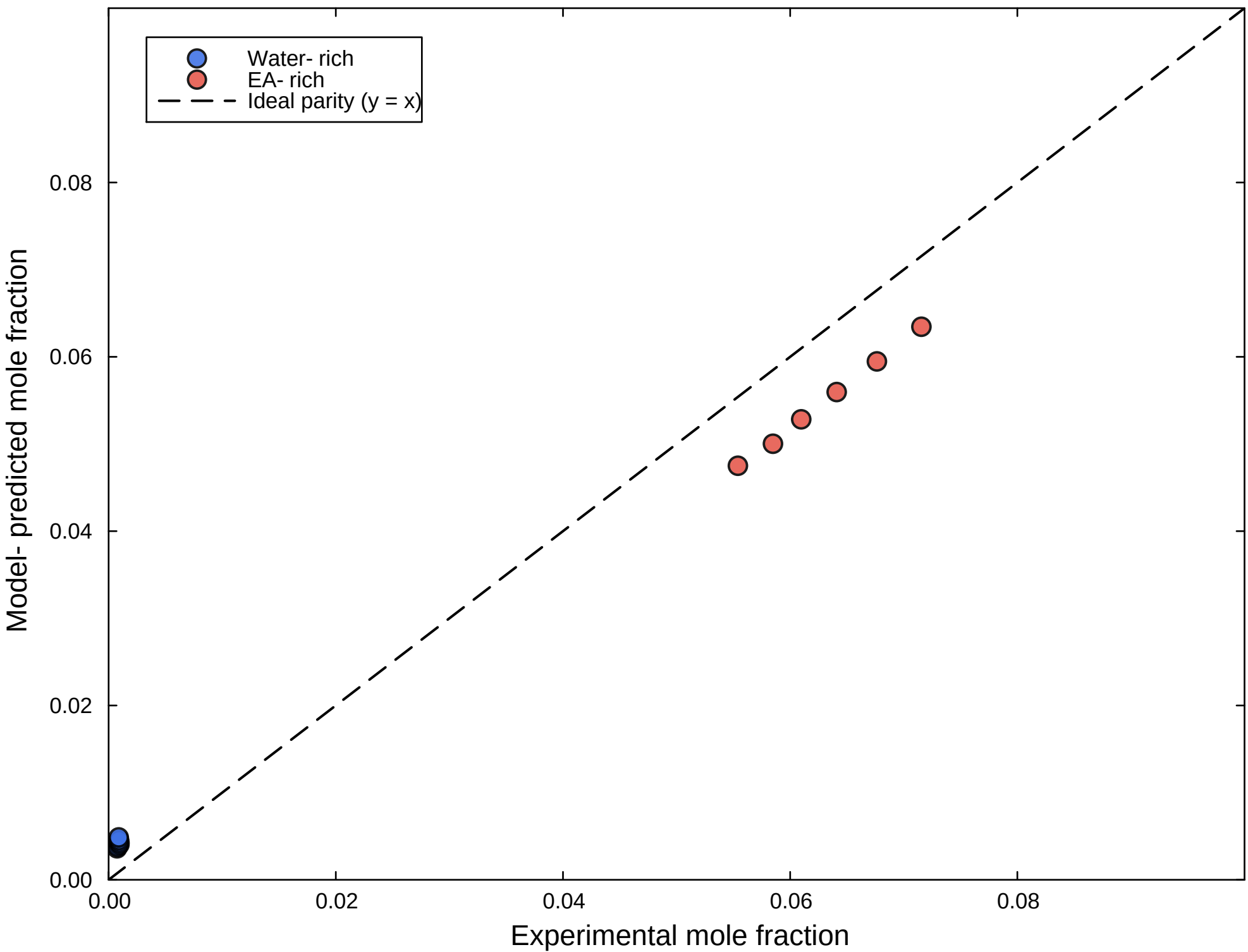
Parity Plot: Furfural Mole Fraction (Model vs Experiment)
