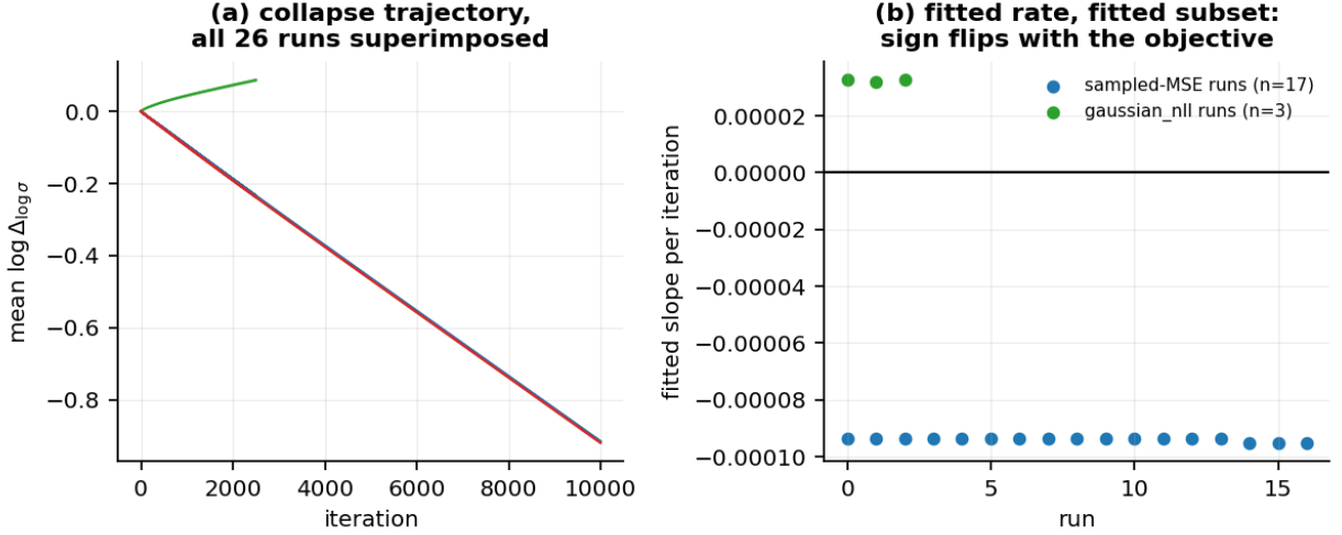
Figure 4: The variance collapse is objective-driven. (a) mean \log \Delta_{\log \sigma} against training iteration for each of the 26 runs of the collapse family, which is every run at the released width. (b) the fitted per-iteration slope for each run, grouped by objective: negative and tightly clustered under sampled MSE, positive under gaussian_nll . The sign flip is the evidence that the objective, not the optimiser or the data, produces it.
