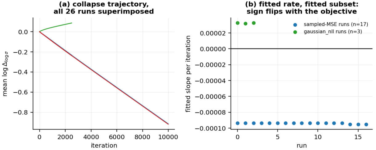
Figure 4: The variance collapse is objective-driven. (a) mean log \Delta_{\log \sigma} against training iteration for every run. (b) the fitted per-iteration slope for each run, grouped by objective: negative and tightly clustered under sampled MSE, positive under gaussian_nll . The sign flip is the evidence that the objective, not the optimiser or the data, produces it.
