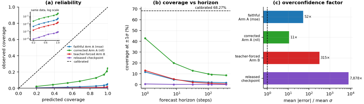
Figure 3: Calibration of all four models on the held-out arena. The released checkpoint trained on these episodes, so for it this arena is in-sample (§3). (a) reliability: observed against predicted coverage, with the calibrated diagonal; the inset repeats the same points with observed coverage on a log scale, where the four models separate. (b) coverage at \pm 1\sigma against forecast horizon, log scale, against the 68.27% a calibrated Gaussian gives. Every curve sits far below the diagonal and falls further with horizon. (c) the overconfidence factor for each model: mean absolute error divided by mean predicted \sigma , log scale, with the dashed line where error equals \sigma .
