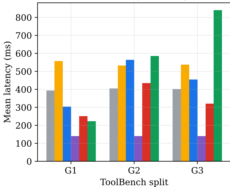
Fig. 4: Per-split breakdown on ToolBench G1/G2/G3 Per-split success (converged) Per-split latency (converged)
