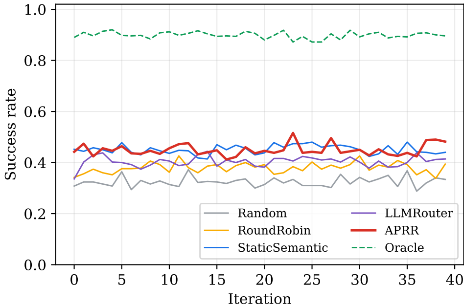
Fig. 1: Convergence of success rate
