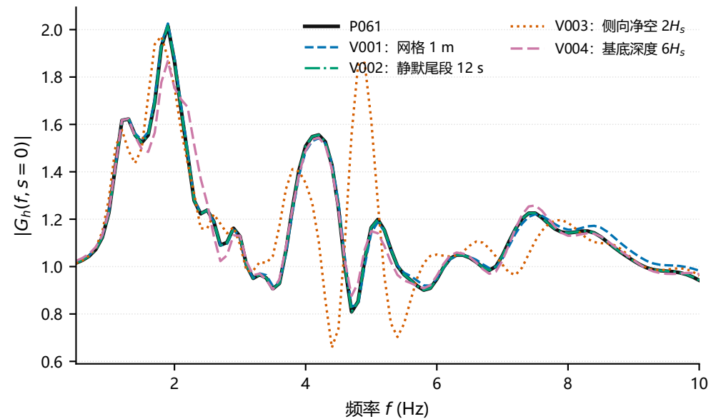
(a) 坡顶复频响应幅值
