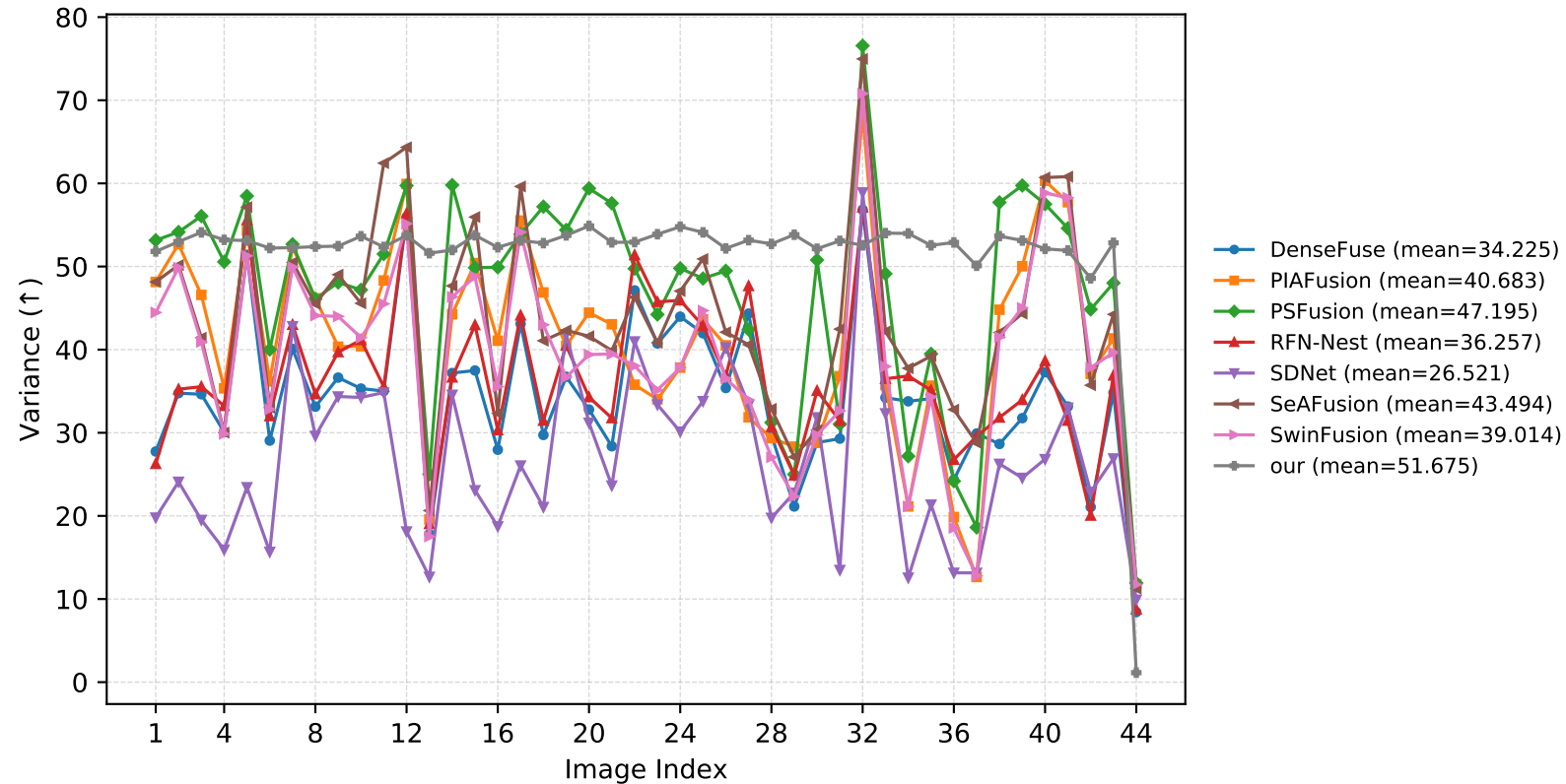
Variance
