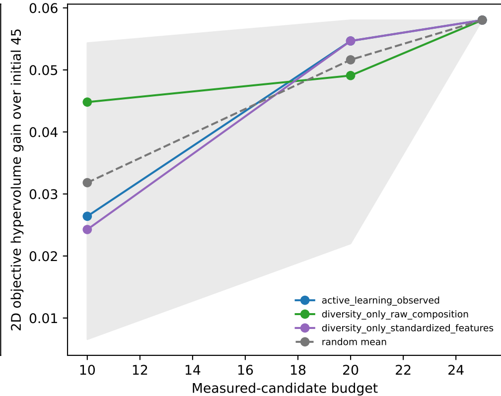
Pareto hypervolume
