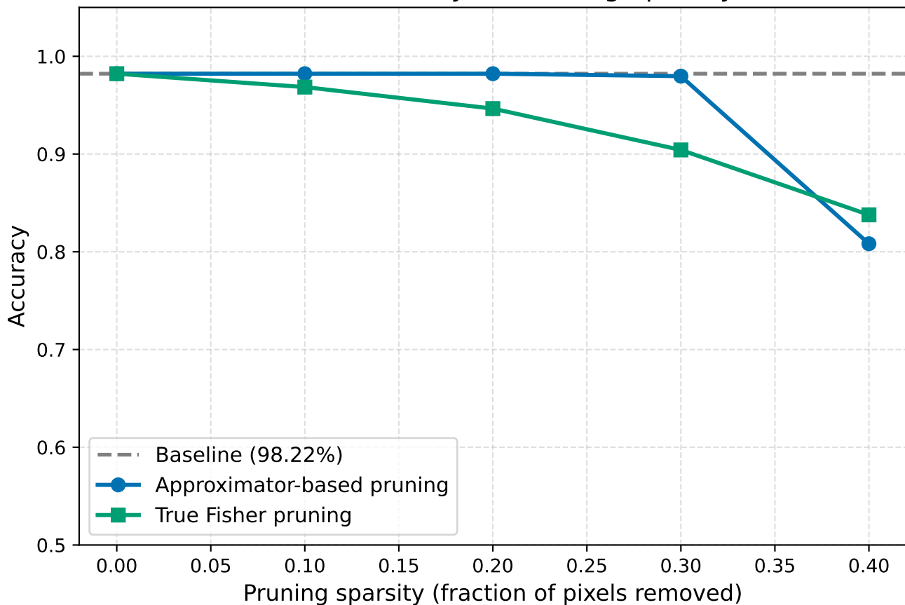
MNIST: Accuracy vs. Pruning Sparsity
