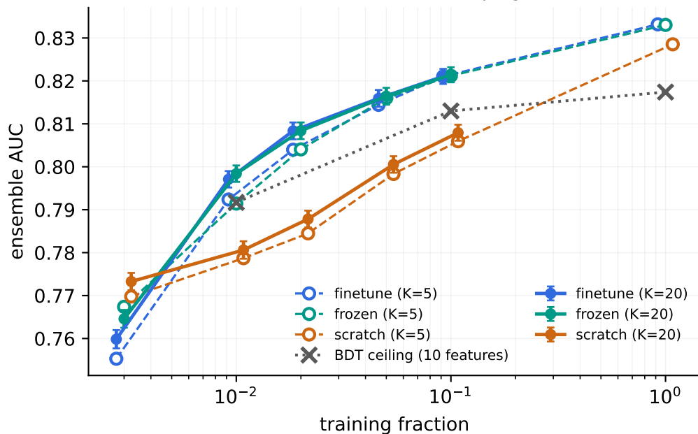
ensemble AUC, both campaigns
