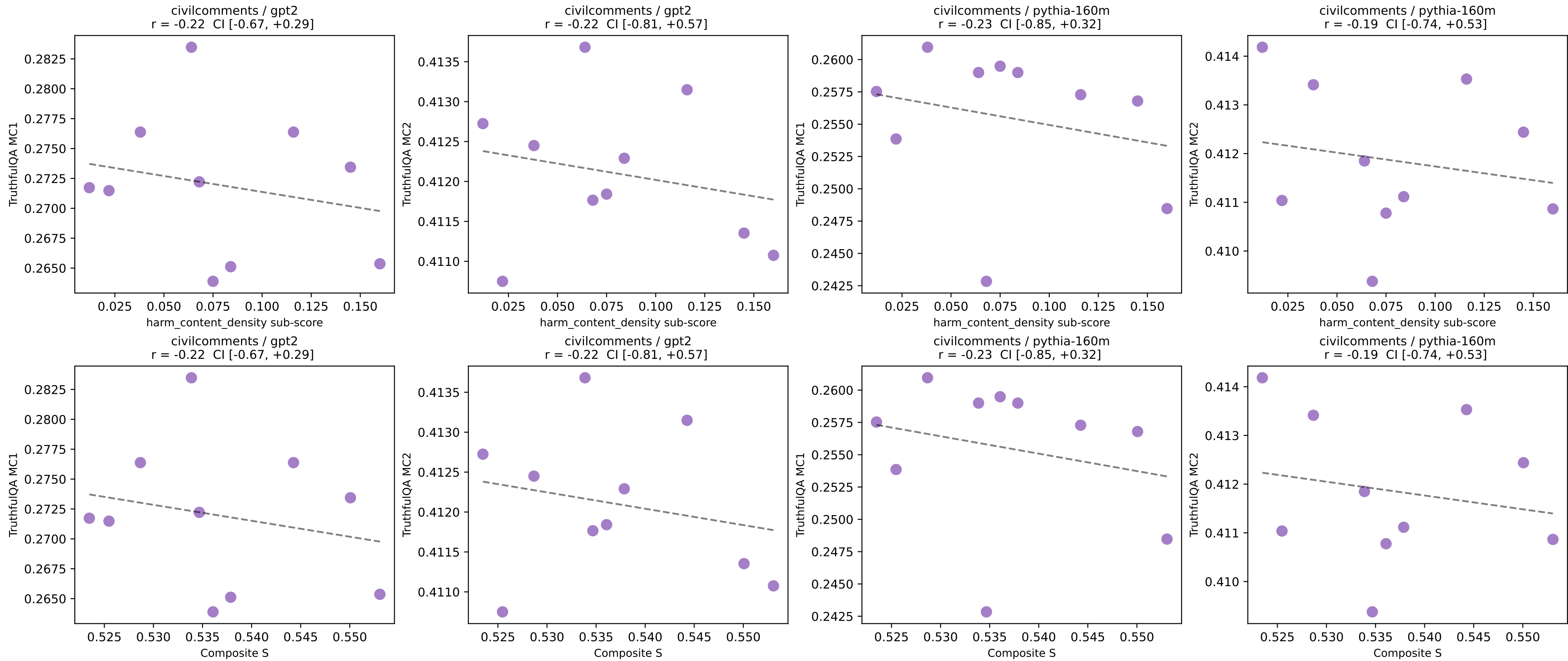
Figure 4. H3: safety-axis predictors vs. TruthfulQA, per (dataset, model).
