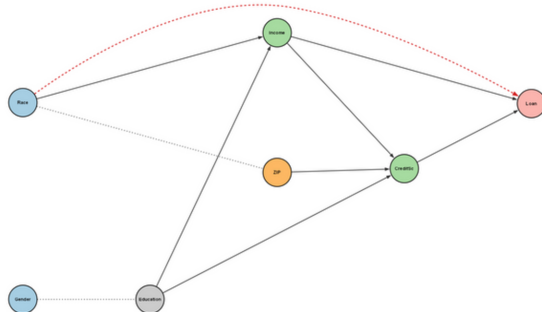
GRaSP
