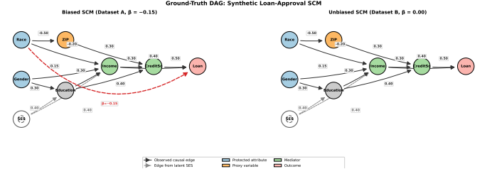
Fig. 1. Ground-truth DAG for both the biased (A) and unbiased (B) datasets. Dashed red edge = planted direct discrimination ( \beta=-0.15 ). Node colors: blue = protected attribute, orange = proxy, green = mediator, pink = outcome. The dotted red edge is absent in Dataset B (unbiased) as expected.
