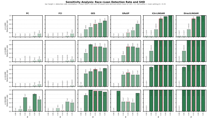
Fig. 2. Sensitivity analysis: Race→Loan detection rate (color intensity) and sample size n (rows), across all algorithms (columns). The bar height encodes detection rate; the annotation within each bar reports the mean SHD ± standard deviation over 20 seeds, capturing the structural accuracy of the recovered graph independently of whether the bias edge was detected.
