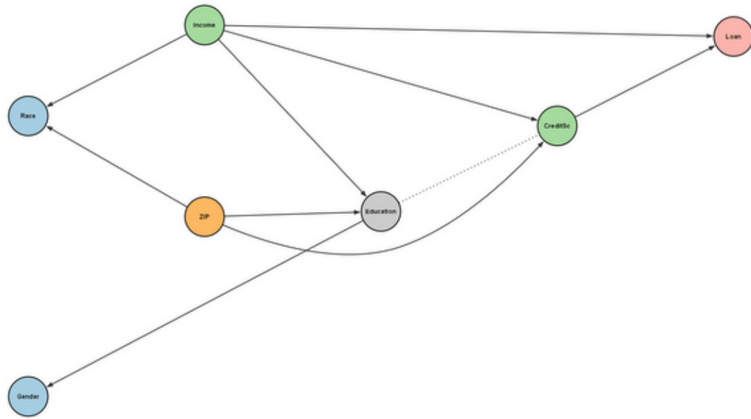
GRaSP
