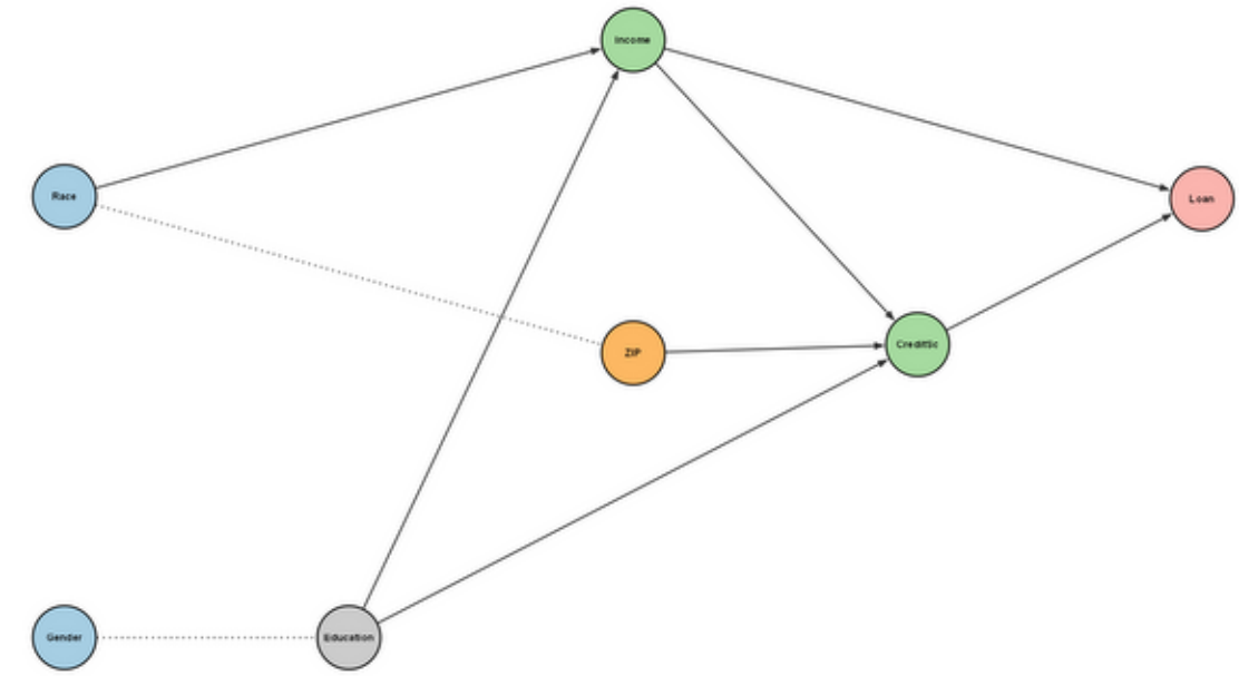
DirectLiNGAM \hat{\beta} = +0.000
