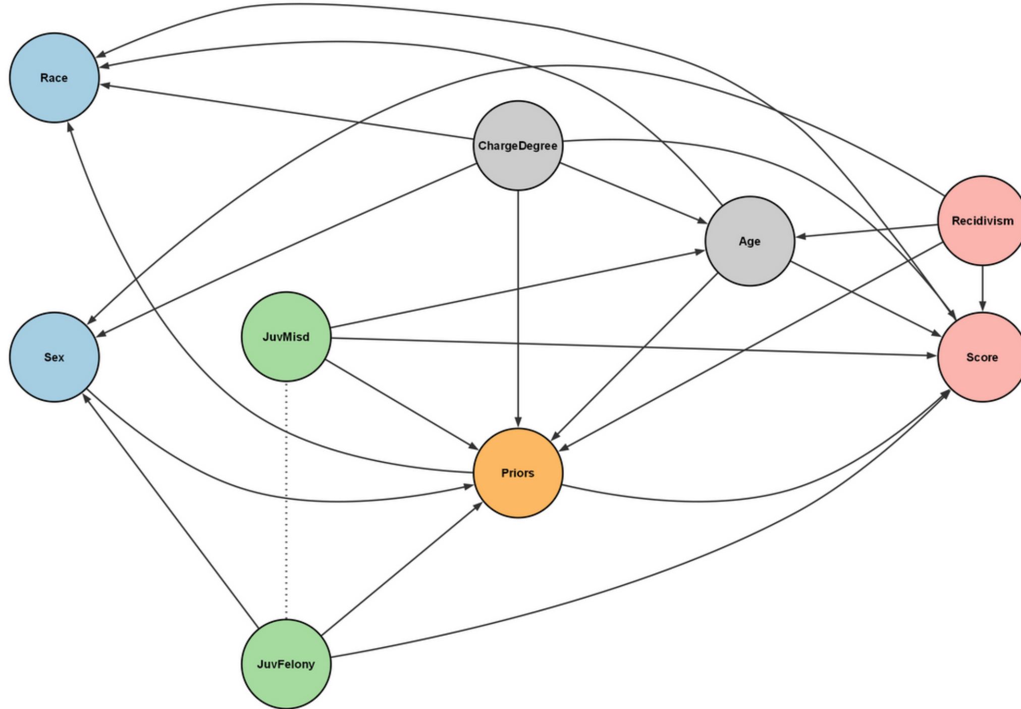
PC on COMPAS (n=9380)
