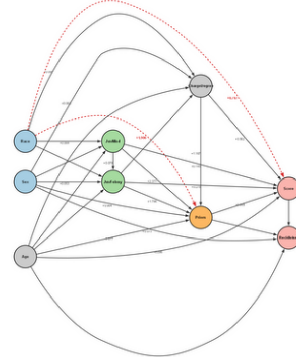
DirectLiNGAM
