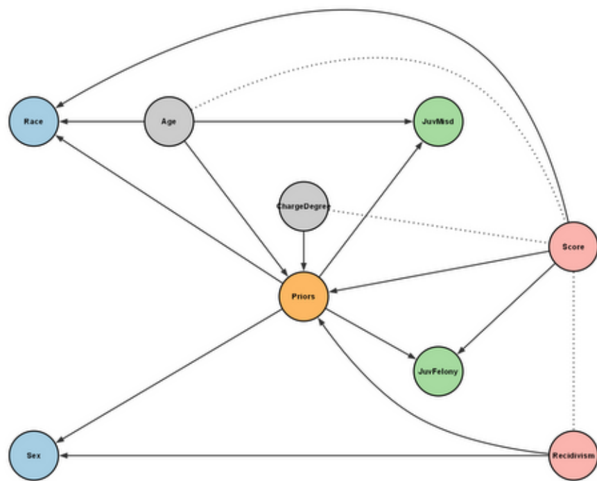
GRaSP
