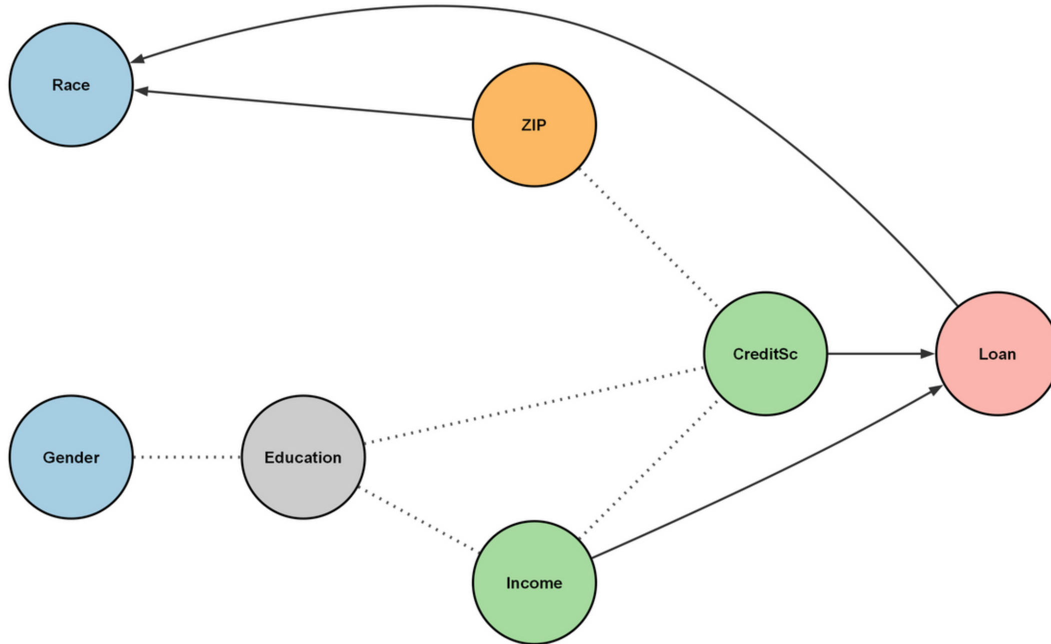
FCI on Biased Dataset ( \beta = -0.15 )
