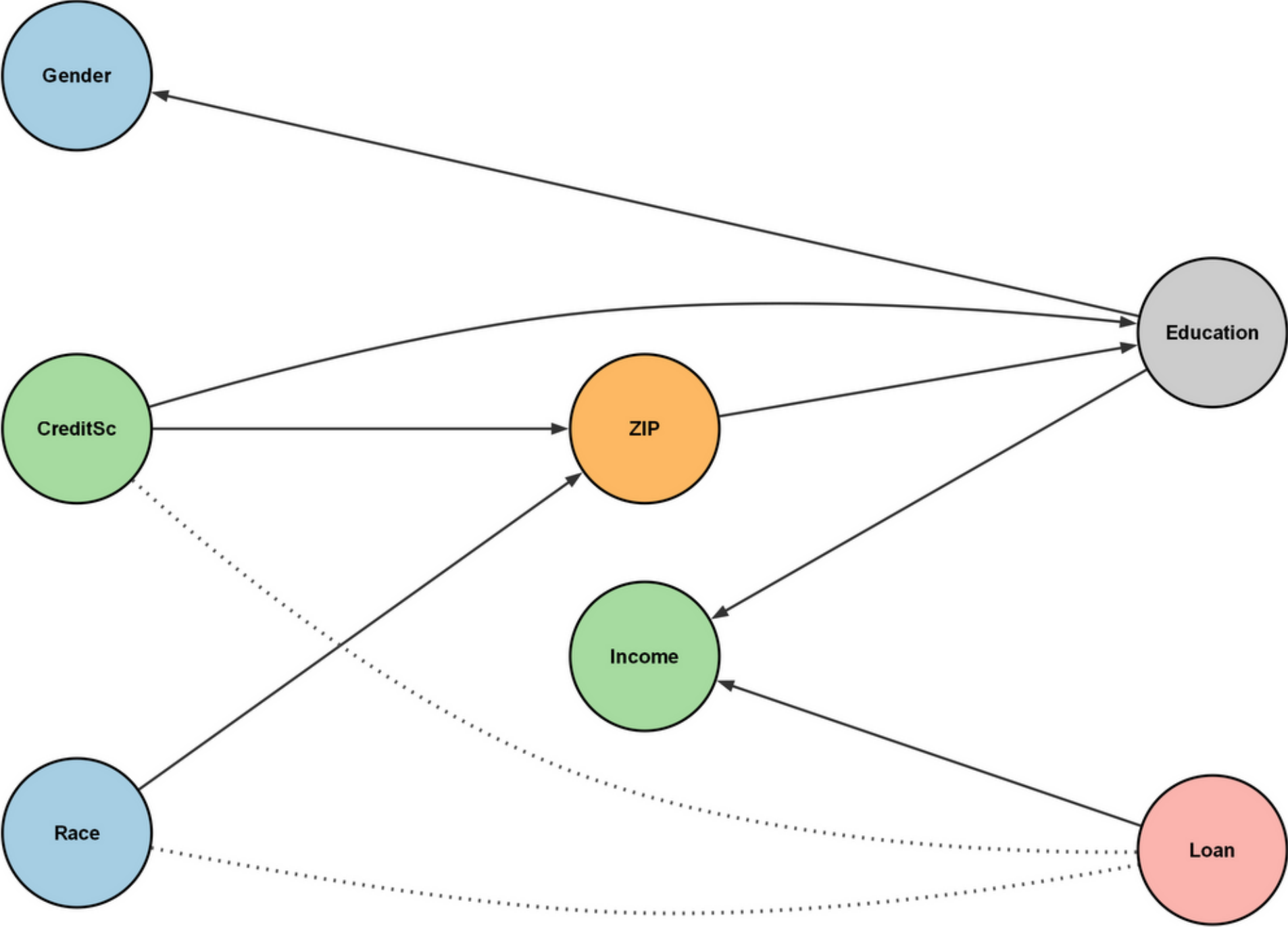
GRaSP on Biased Dataset ( \beta = -0.15 )
