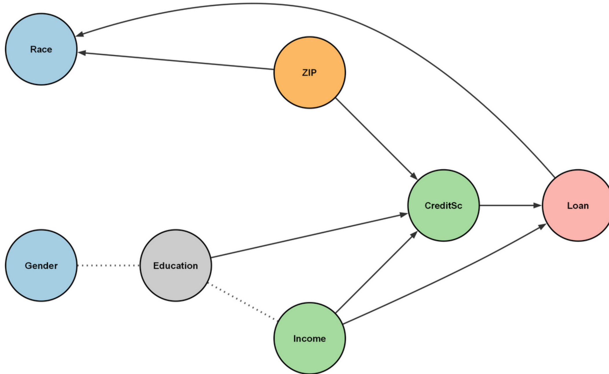
PC on Biased Dataset ( \beta = -0.15 )
