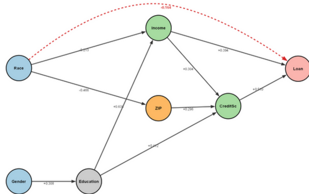
ICA-LiNGAM
