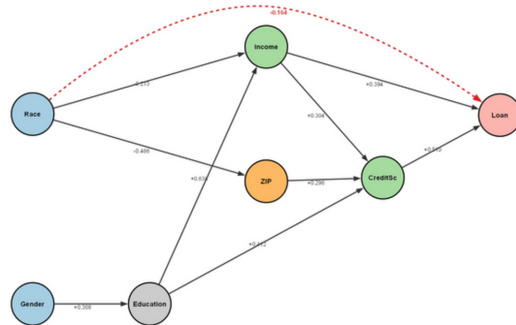
DirectLiNGAM
