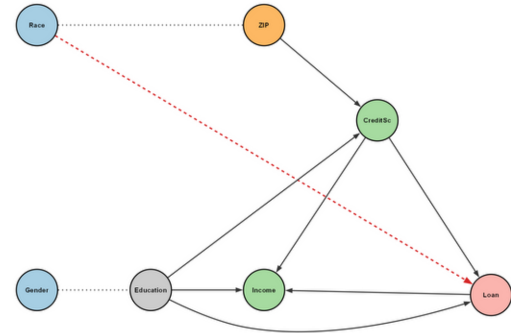
DirectLiNGAM
