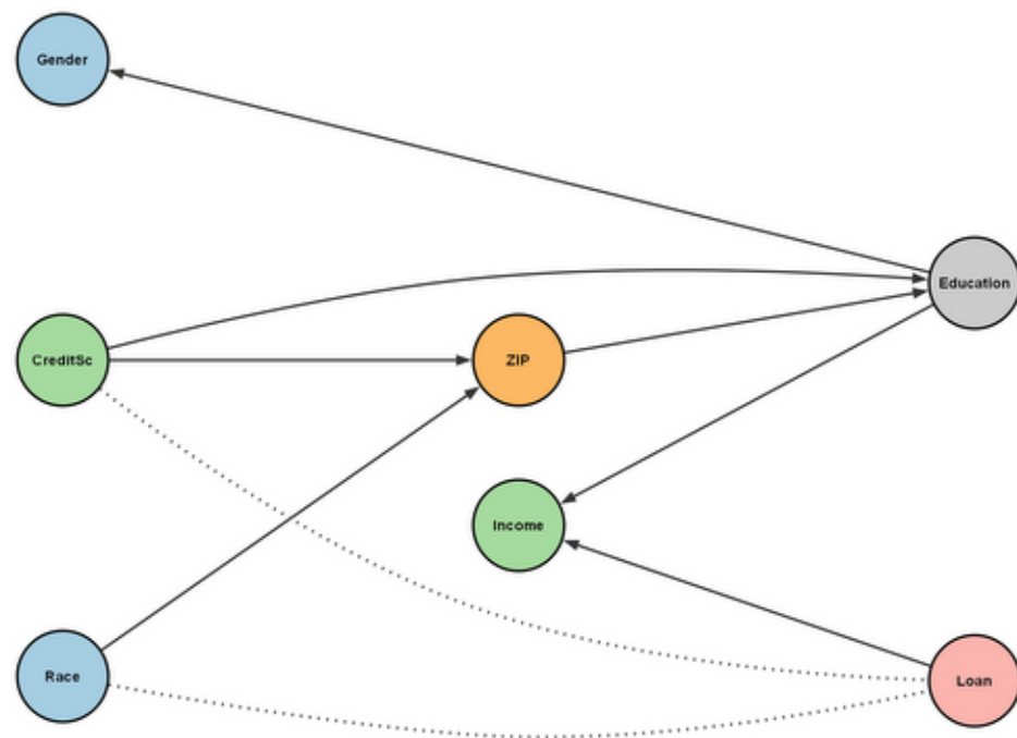
GRaSP
