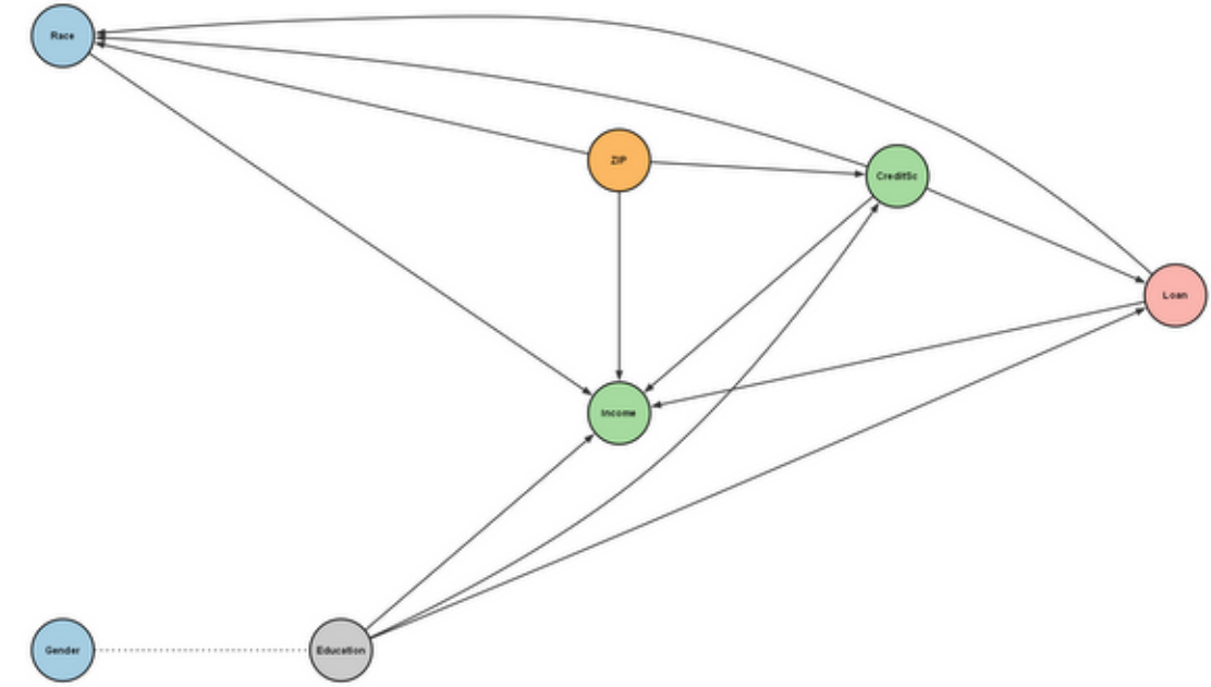
DirectLiNGAM \hat{\beta} = -0.107
