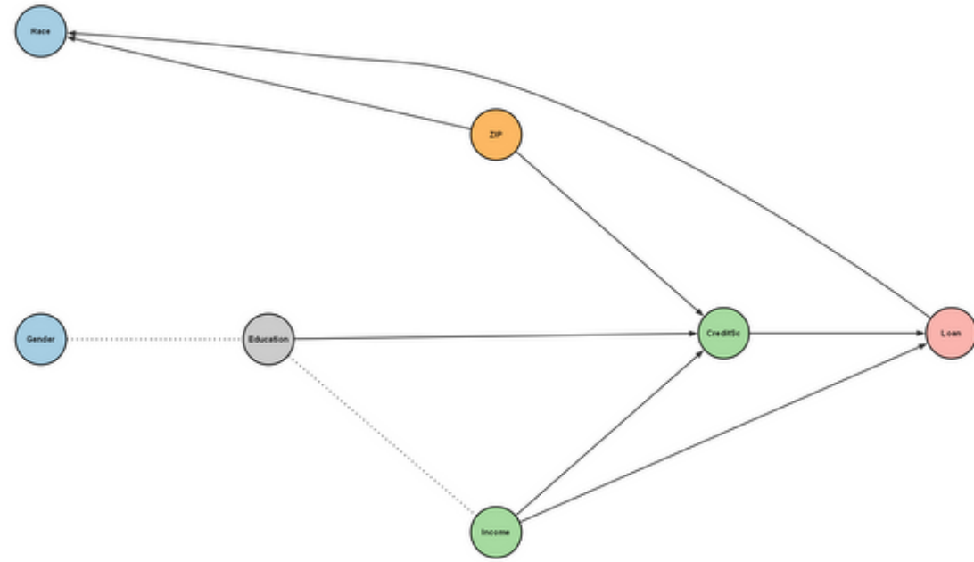
GRaSP
