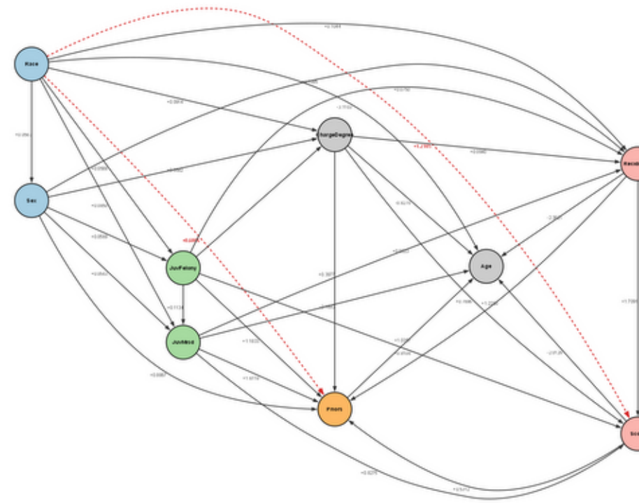
ICA-LiNGAM
