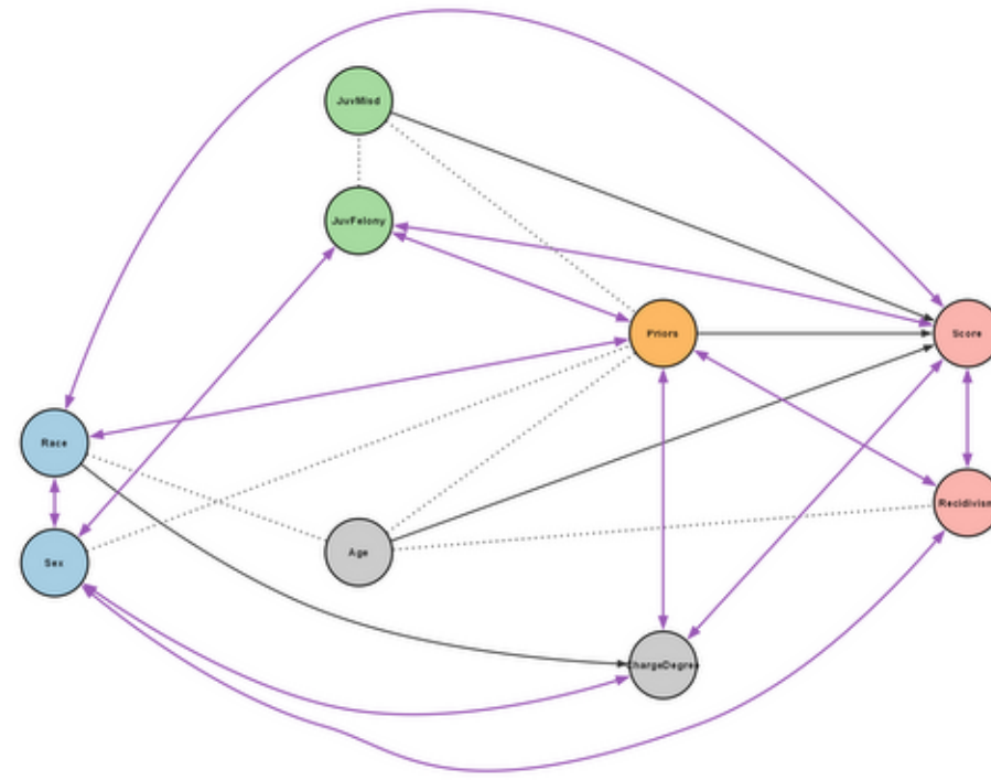
ICA-LiNGAM
