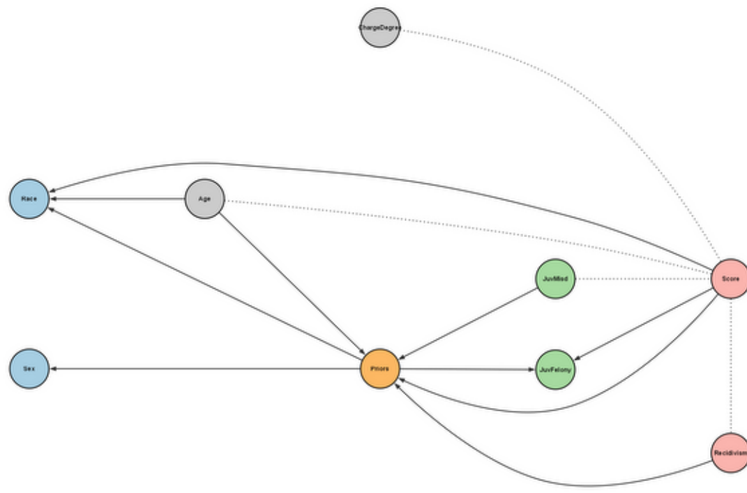
GRaSP
