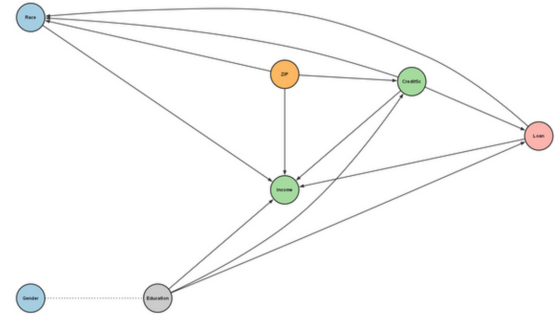
DirectLiNGAM \hat{\beta} = -0.107
