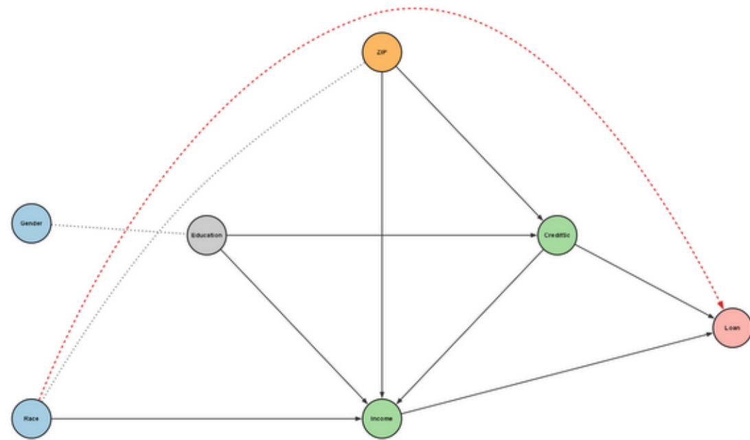
GRaSP
