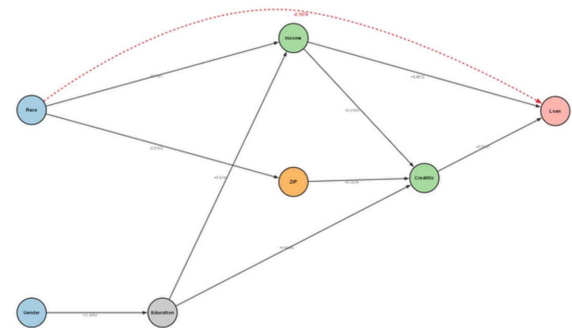
DirectLiNGAM \hat{\beta} = -0.107
