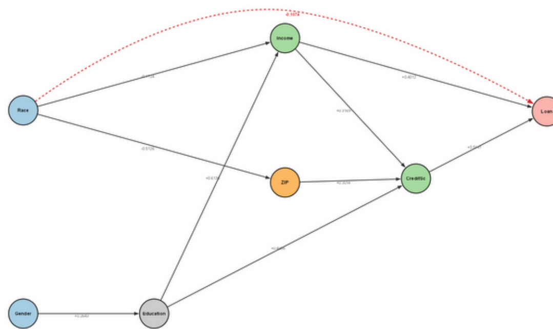
ICA-LiNGAM \hat{\beta} = -0.107
