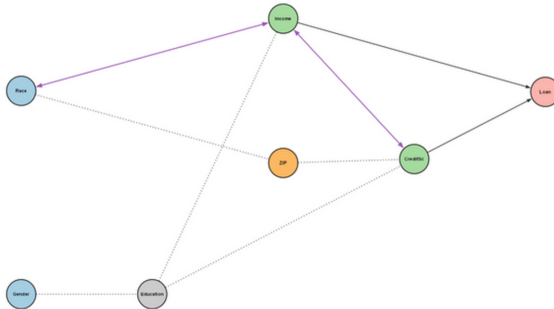
ICA-LiNGAM
