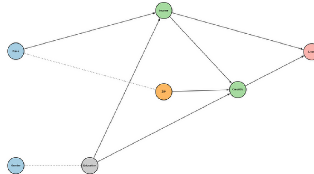
DirectLiNGAM
