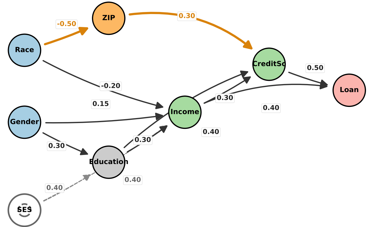
Unbiased SCM (Dataset B, \beta = 0.00 )
