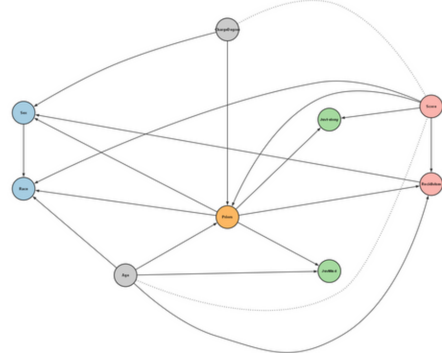
DirectLiNGAM \hat{\beta}=+0.5167
