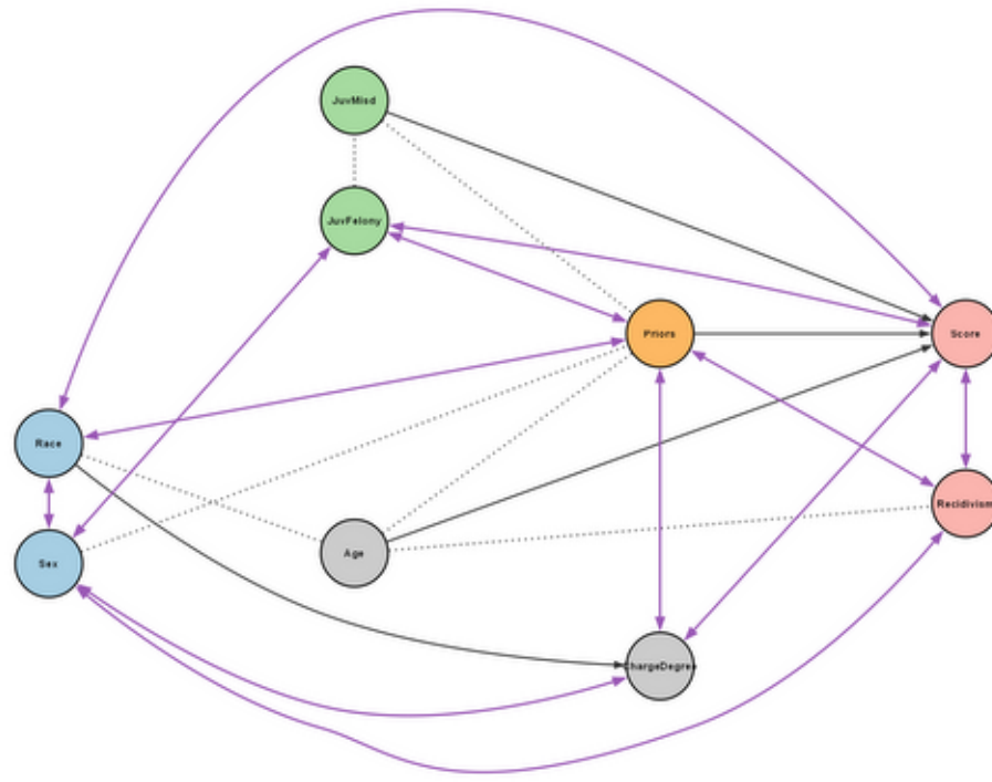
ICA-LiNGAM \hat{\beta}=+1.2105
