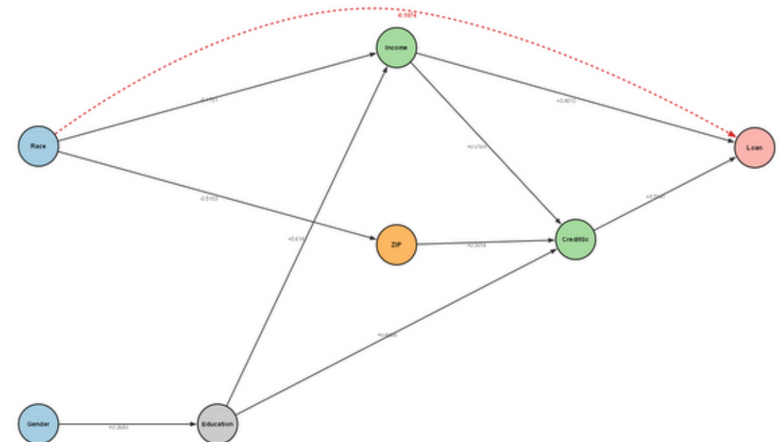
DirectLiNGAM \hat{\beta}=-0.107
