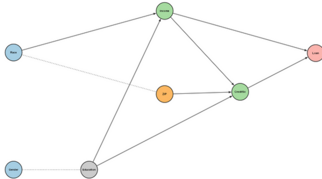
GRaSP
