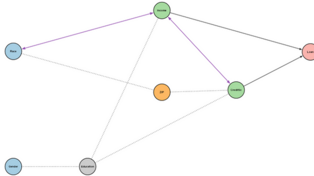
ICA-LiNGAM \hat{\beta} = +0.000
