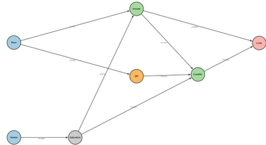
DirectLiNGAM \hat{\beta} = +0.000
