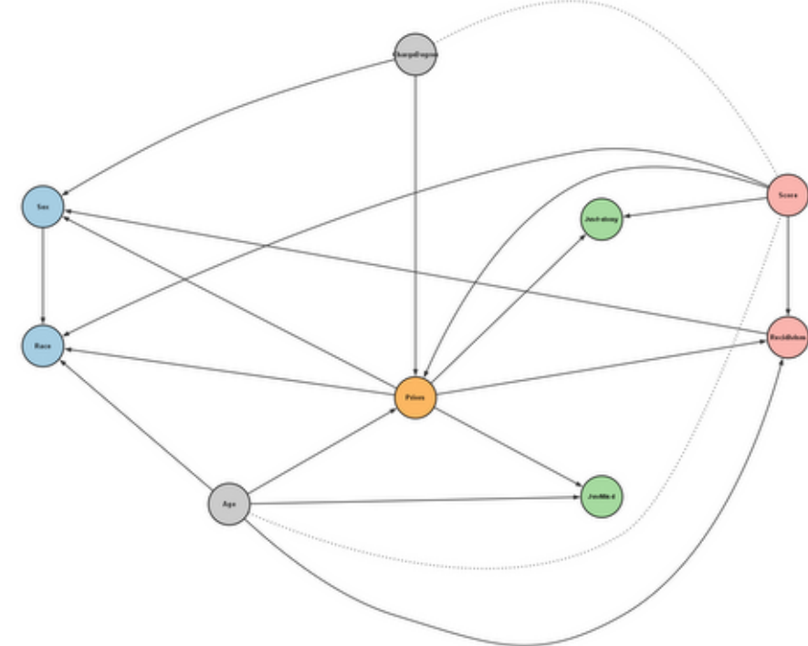
DirectLiNGAM
