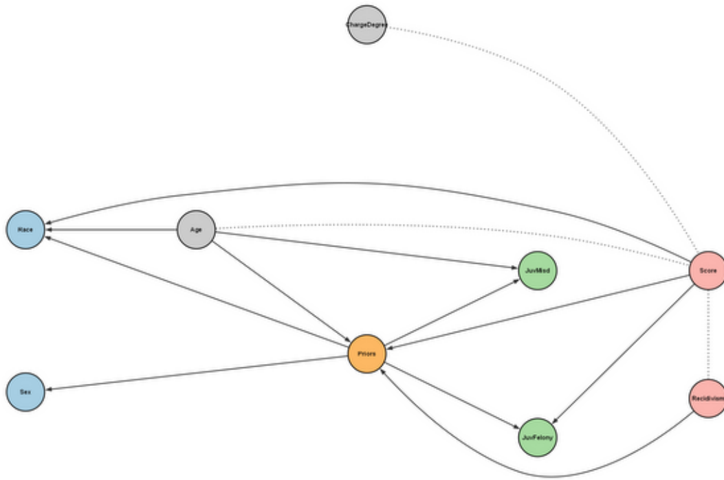
GRaSP
