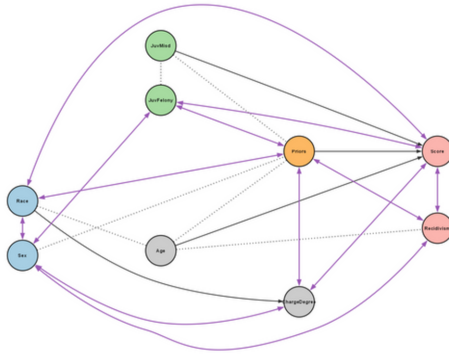
ICA-LiNGAM
