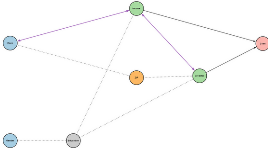
ICA-LiNGAM \hat{\beta} = +0.000
