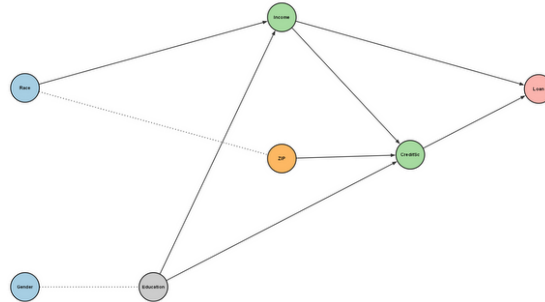
DirectLiNGAM \hat{\beta} = +0.000
