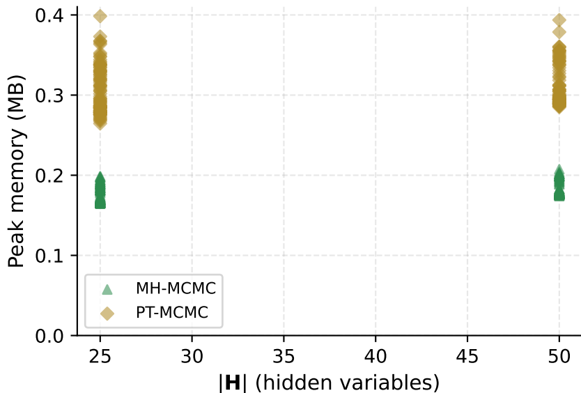
MCMC memory vs. |\mathbf{H}|
