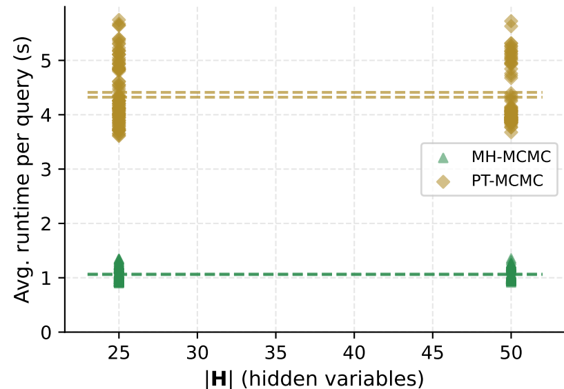
MCMC runtime vs. |\mathbf{H}|
