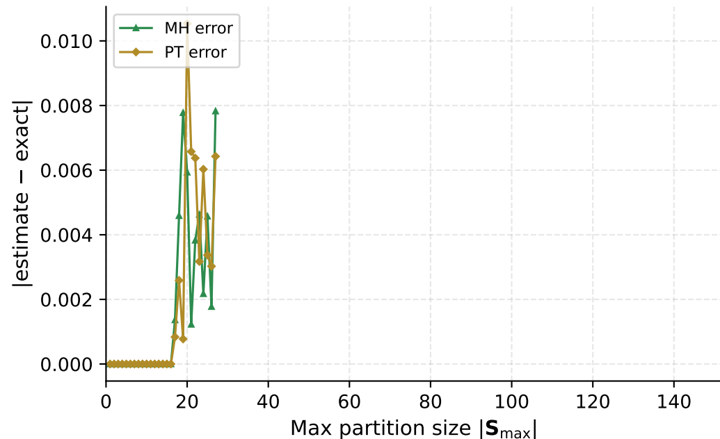
MCMC absolute error (where exact ran)
