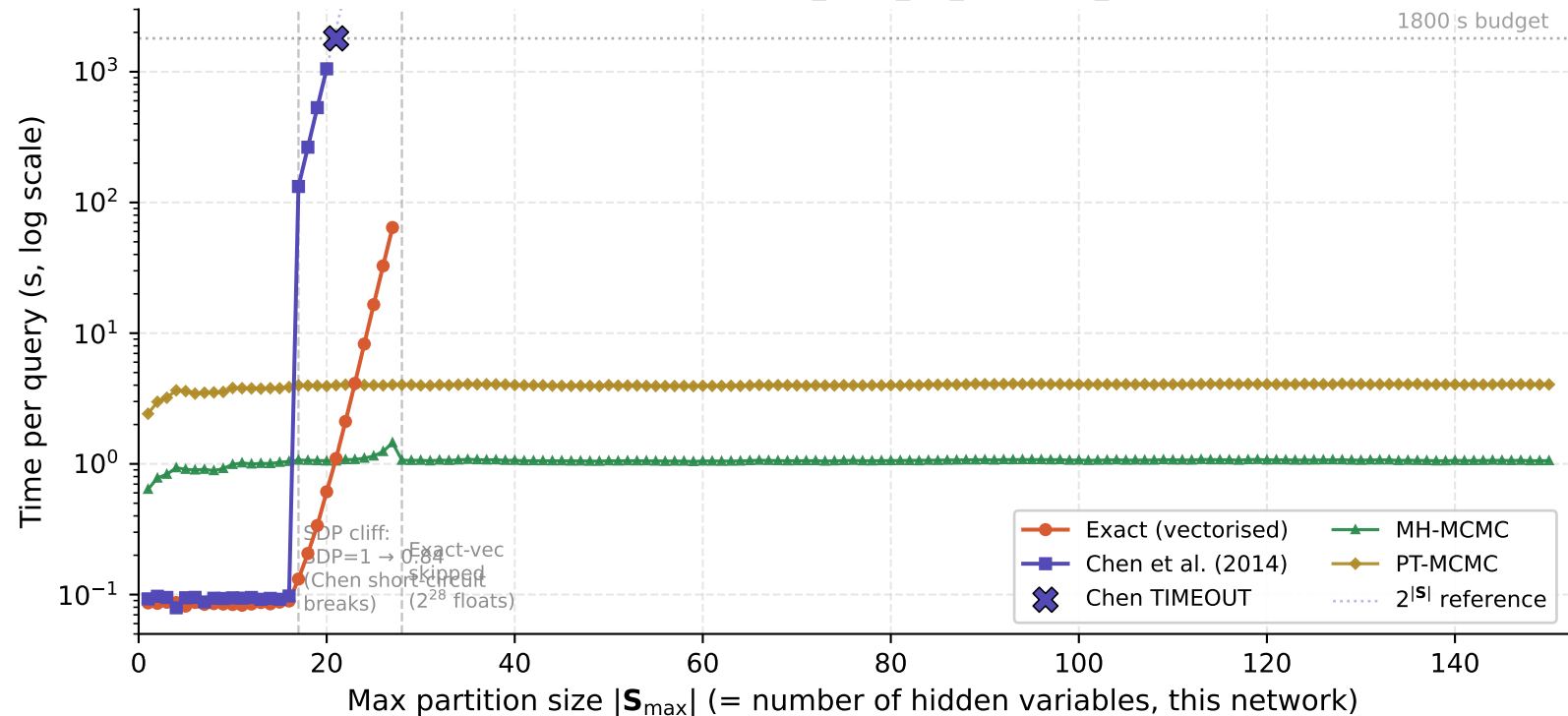
Runtime on growing partition · bn_n200_w2_uncertain_strong · 150 steps
