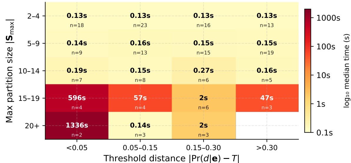
Median Chen runtime ( \log_{10} seconds)
