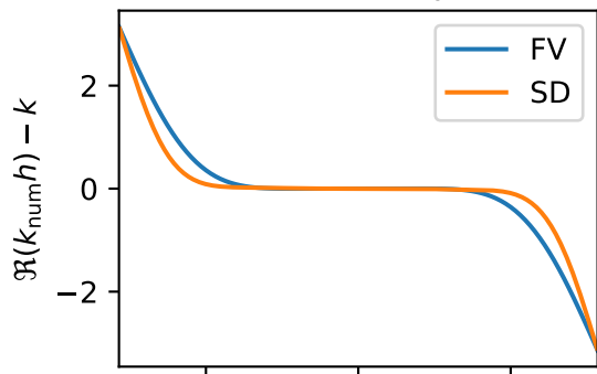
Fourth-order upwind
