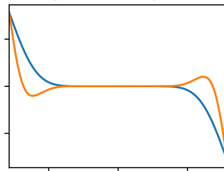
Eighth-order upwind
