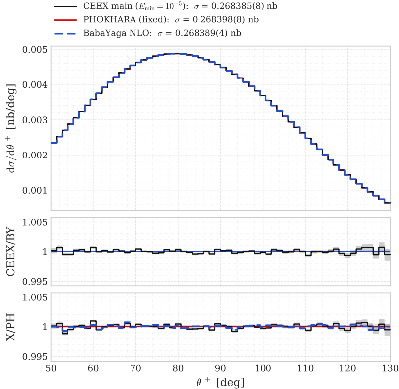
Figure 3: After the fix. As Figure 2, with the fixed PHOKHARA (1000 \times 5M, w = 10^{-5} ) in red and as the denominator of the bottom panel. The tilt is gone.
