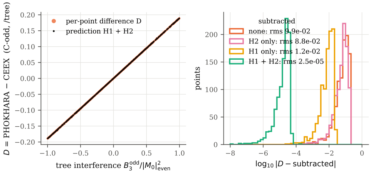
Figure 6: Per-point comparison, 988 one-photon points. Left: the C -odd difference D against the tree interference, with the H1+H2 prediction. Right: \log_{10} |D - \text{subtracted}| for no subtraction, H1, H2 and H1+H2.
