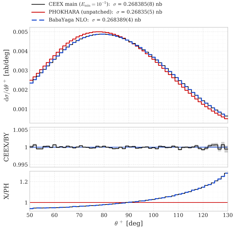
Figure 2: Before the fix. Top: d\sigma/d\theta^+ from CEEX ( E_{\min} = 10^{-5} GeV, 199 \times 5 \times 1M, black), the unpatched PHOKHARA (300 \times 500k, red) and BabaYaga (blue, dashed), 60 bins; the legend gives each total cross section. Middle: CEEX/BabaYaga (CEEX/BY). Bottom: CEEX and BabaYaga over PHOKHARA (X/PH). CEEX and BabaYaga agree; PHOKHARA is tilted.
