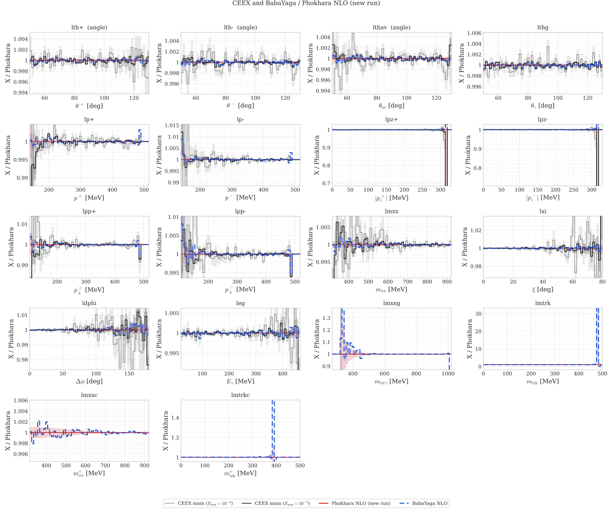
Figure 7: After the fix: every observable, CEEX (more1M at E_{\min} = 10^{-5} , prod500k at 10^{-4} ) and BabaYaga over the fixed PHOKHARA ( 1000 \times 5M ).
