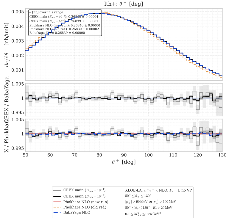
Figure 6: After the fix: as Figure 1, with the fixed PHOKHARA ( 1000 \times 5\text{M} , w = 10^{-5} ) as the denominator and CEEX more1M ( 144 \times 5 \times 1\text{M} ) at E_{\text{min}} = 10^{-5} , prod500k at 10^{-4} . The tilt is gone.
