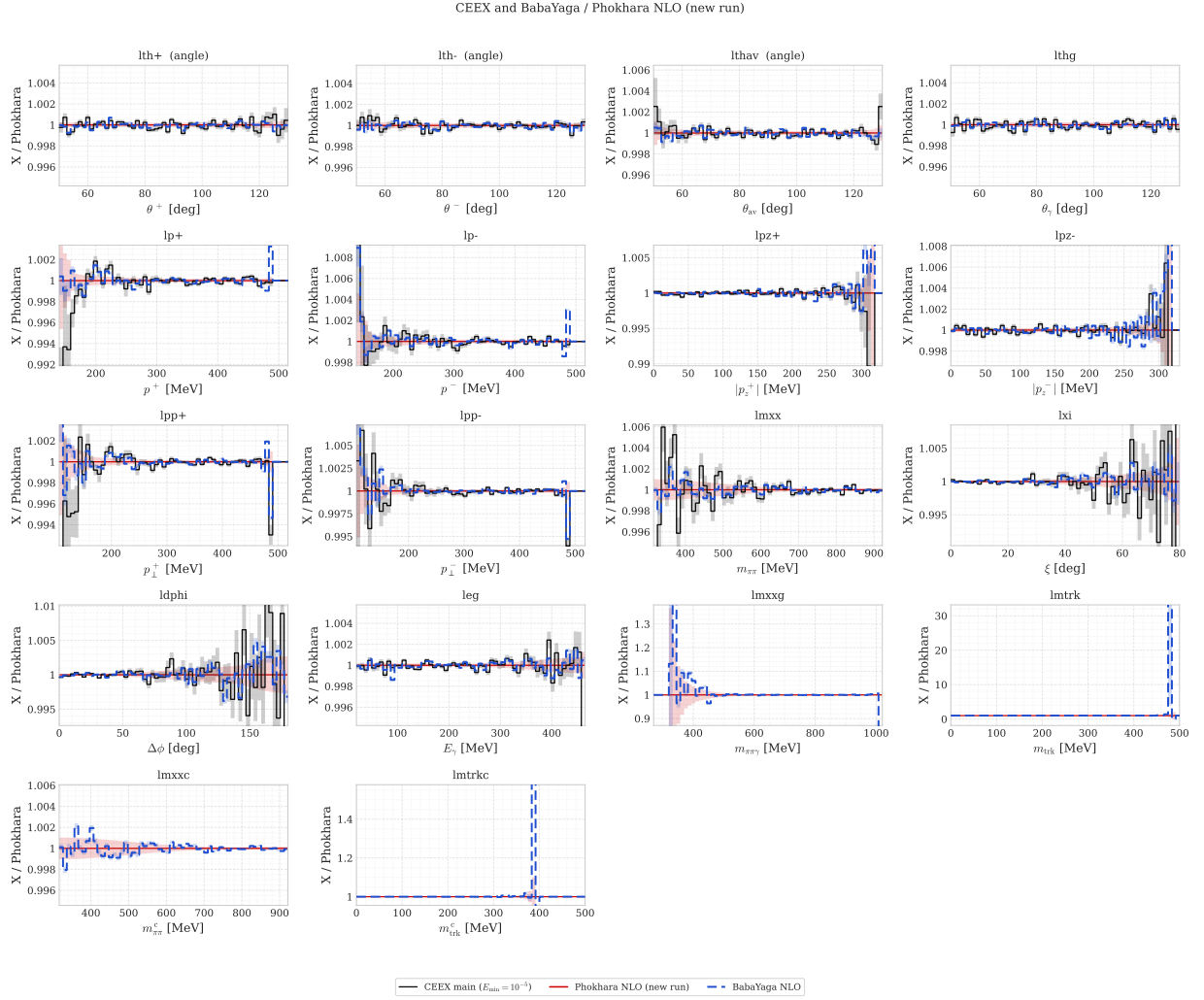
Figure 7: After the fix: every observable, CEEX (more1M, E_{\min} = 10^{-5} GeV) and BabaYaga over the fixed PHOKHARA ( 1000 \times 5M ).
