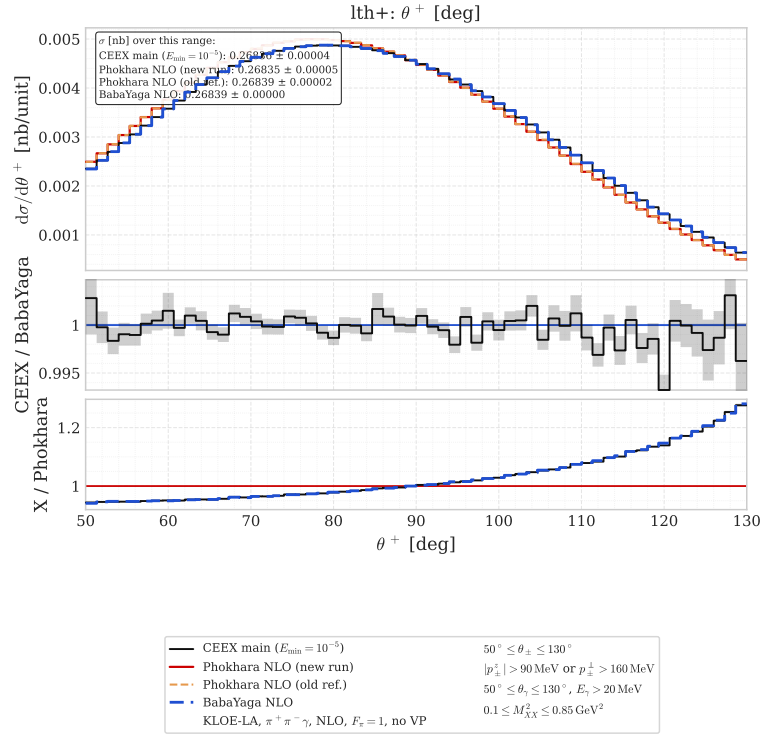
Figure 1: Before the fix (prod500k): d\sigma/d\theta^+ , CEEX/BabaYaga, and CEEX and BabaYaga over PHOKHARA (60 bins). CEEX ( E_{\min} = 10^{-5} GeV, black) and BabaYaga (blue) agree; PHOKHARA (red) is tilted.
