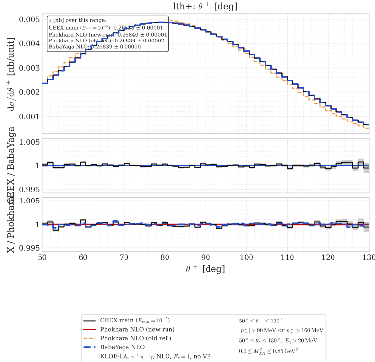
Figure 7: After the fix: as Figure 2, with the fixed PHOKHARA (1000 \times 5M, w = 10^{-5} ) as the denominator and CEEX more1M (199 \times 5 \times 1M, E_{\text{min}} = 10^{-5} GeV). The tilt is gone.
