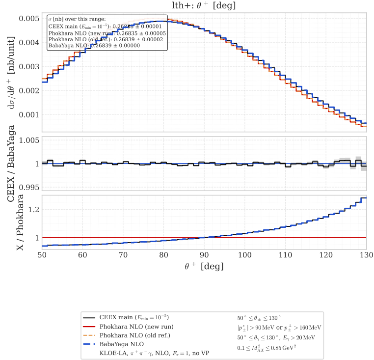
Figure 2: Before the fix: unpatched PHOKHARA (300×500k) against CEEEX more1M (199×5×1M): d\sigma/d\theta^+ , CEEEX/BabaYaga, and CEEEX and BabaYaga over PHOKHARA (60 bins). CEEEX ( E_{\min} = 10^{-5} GeV, black) and BabaYaga (blue) agree; PHOKHARA (red) is tilted.
