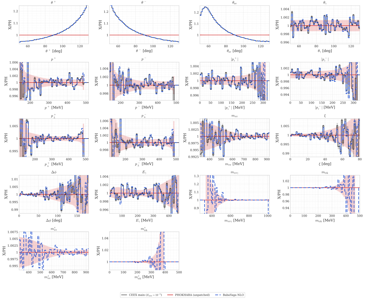
Figure 5: Before the fix: every observable, CEEX and BabaYaga over PHOKHARA. Only \theta^+ , \theta^- and \theta_{\text{av}} are off; the spikes in M_{\pi\pi\gamma} and M_{\text{trk}} are empty tail bins.
