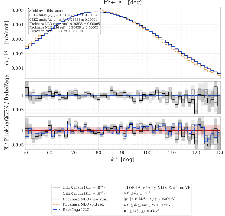
Figure 6: After the fix: as Figure 1, with the fixed PHOKHARA (300×500k, w = 10^{-5} ). The tilt is gone.
