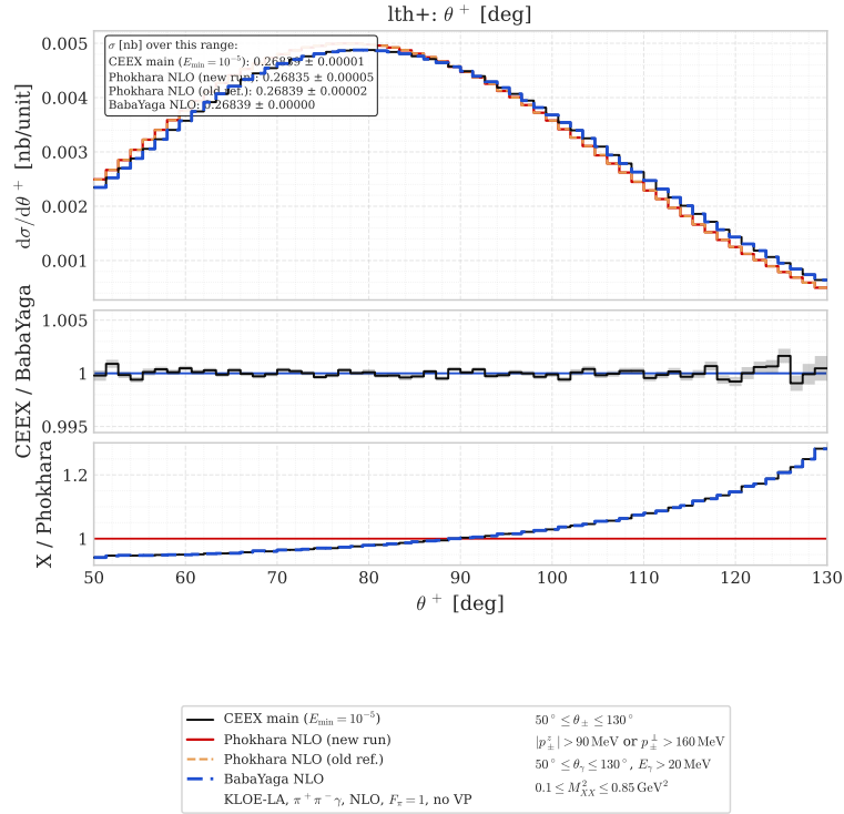
Figure 1: Before the fix: unpatched PHOKHARA (300 \times 500k) against CEEX more1M (148 \times 5 \times 1M): d\sigma/d\theta^+ , CEEX/BabaYaga, and CEEX and BabaYaga over PHOKHARA (60 bins). CEEX ( E_{\min} = 10^{-5} GeV, black) and BabaYaga (blue) agree; PHOKHARA (red) is tilted.
