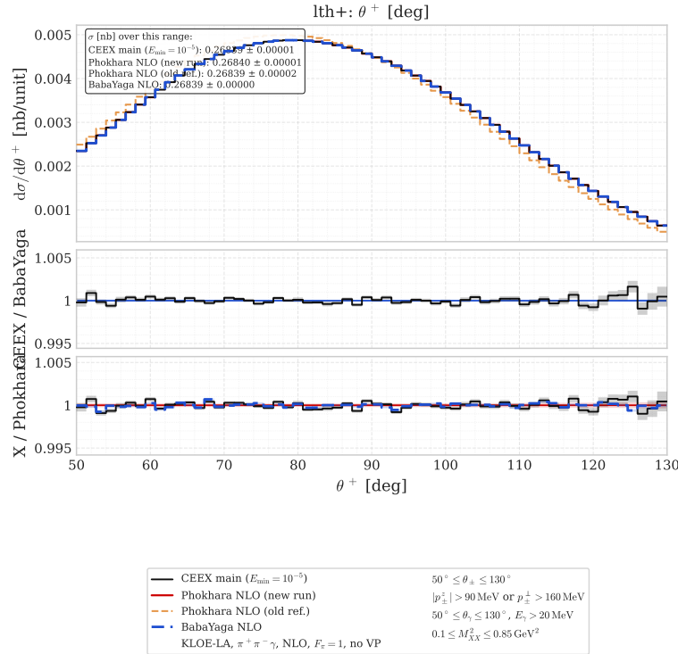
Figure 6: After the fix: as Figure 1, with the fixed PHOKHARA (1000 \times 5M, w = 10^{-5} ) as the denominator and CEEX more1M (148 \times 5 \times 1M, E_{\text{min}} = 10^{-5} GeV). The tilt is gone.
