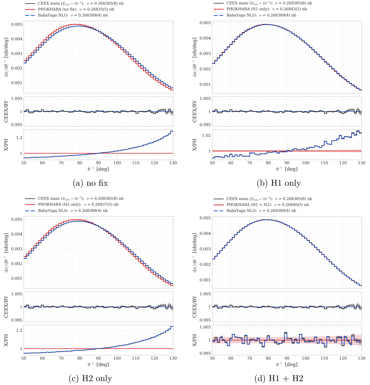
Figure 6: Each fix alone. As Figure 2, with PHOKHARA (300×500k, w = 10^{-5} , red) built (a) without either fix, (b) with H1 only, (c) with H2 only and (d) with both. The bottom panels (CEE and BabaYaga over PHOKHARA) have different vertical scales. The ratio runs from 0.95 to 1.28 in (a), to 1.23 in (c) and only to 1.02 in (b); it is flat only in (d).
