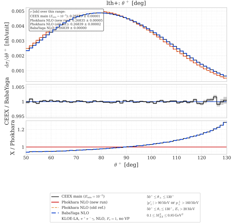
Figure 1: Before the fix: unpatched PHOKHARA (300×500k) against CEEEX more1M (148×5×1M): d\sigma/d\theta^+ , CEEEX/BabaYaga, and CEEEX and BabaYaga over PHOKHARA (60 bins). CEEEX ( E_{\min} = 10^{-5} GeV, black) and BabaYaga (blue) agree; PHOKHARA (red) is tilted.
